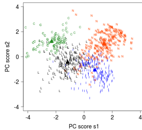
Figure 2: Scatterplot of the values of the first two PC scores s_1 , s_2 as in eq.(1). Speaker group membership is indicated with I(Italian), N(Dutch), L(learners) C(Confederate) labels are marked with a triangle.
