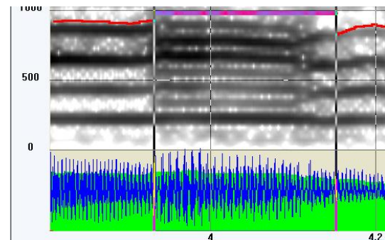
Figure 7. A clear example of a modal to creaky transition, with a detected creaky index of 7/4 (female voice).
