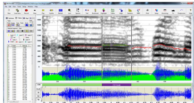
Figure 5. Example of detection of a creaky segment (female voice)
