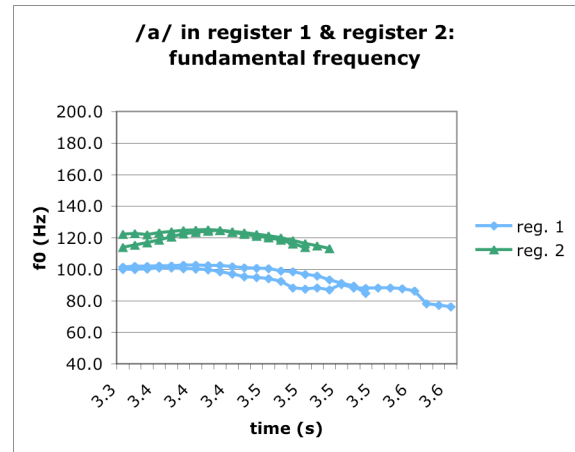
Figure 2. F0 traces for four /a/ tokens; two in register 1 /luwat/ ‘mangrove worm’ and two in register 2 /luwət/ ‘front’. Register 2 is seen to be higher than register 1. The latter was also 70.5ms. longer (cf. Table 4.).
