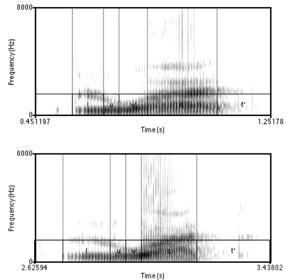
Figure 1. Spectrogram of /luwat/ ‘mangrove worm’ (top), showing the register 1 vowel /a/; and /luwət/ ‘front’, showing the register 2 vowel /a/ (below). Less clearly defined formants, and vertical striations, particularly in the first part, can be seen for register 2.
