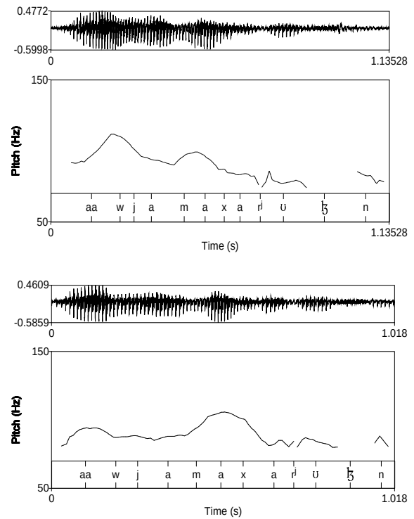
Figure 1: Tonal courses of the sentences aaw jama xar'uʒn “Father herds goats” uttered with focal accent on the first word (top) and on the second word (bottom).
