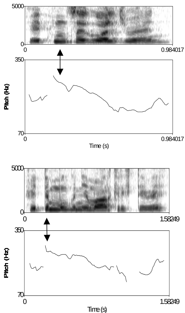
Figure 5: Spectrogram and F0 courses of the utterances xity ts'ag'ht pult' pain? (above) and xity mongni mark xirgt'he wee? (below). /xity/ is realised as [xityŋ] and [xitəm], respectively. The arrow shows the focal H, timed with [ŋ] in the first utterance and with [ə] in the second one.
